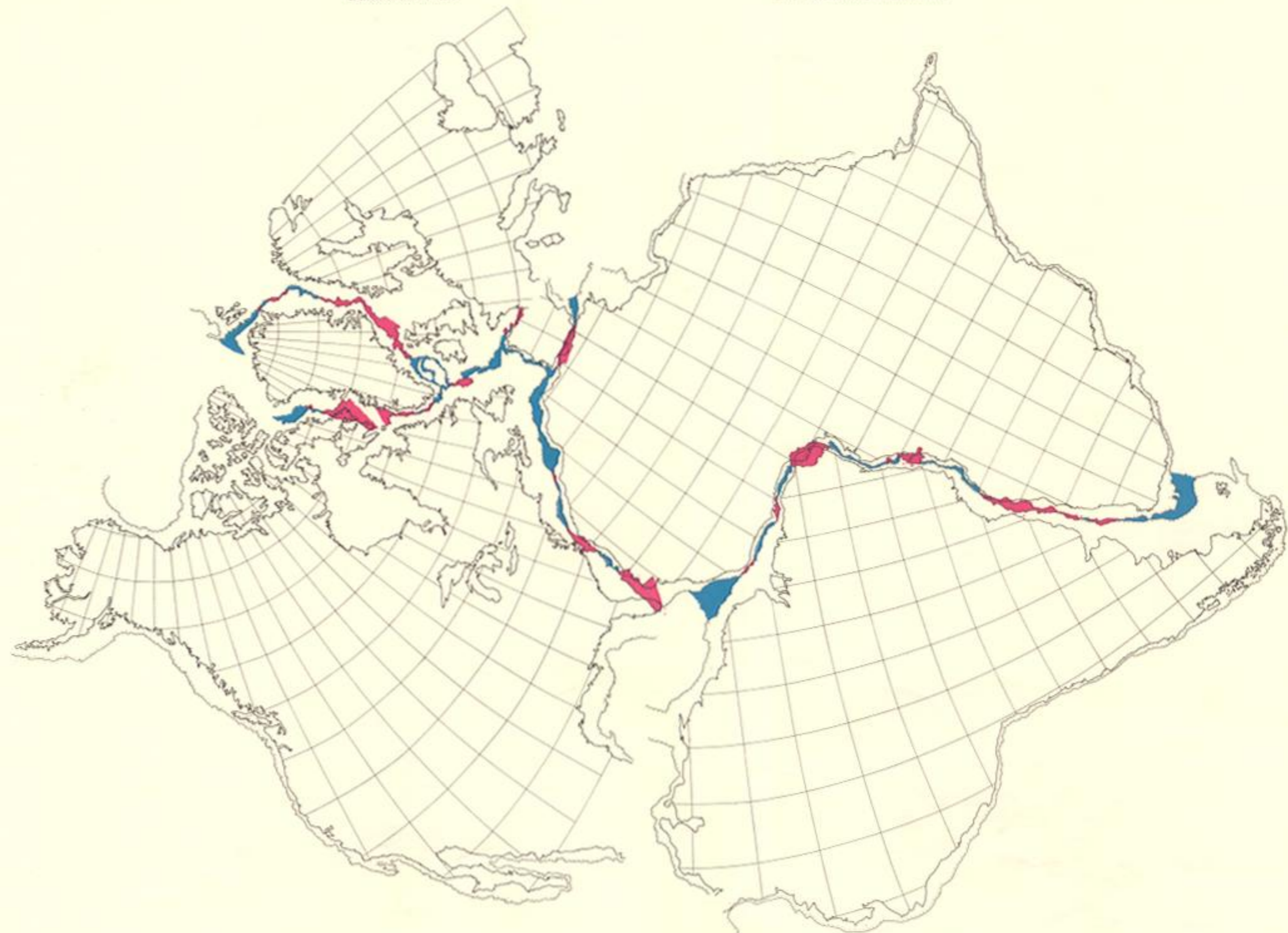
FIGURE 8. Fit of all the continents around the Atlantic at the 500 fm. contour, transverse Mercator projection.
