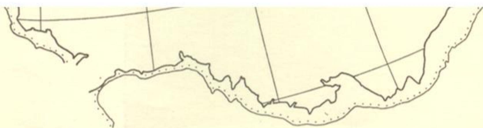
Atlantic at the 500 fm. contour, transverse Mercator projection.
