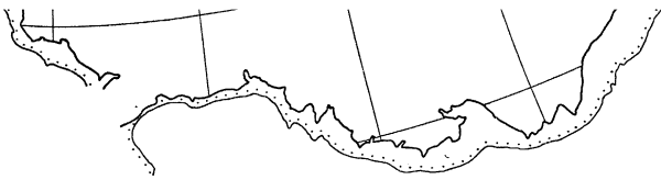
Atlantic at the 500 fm. contour, transverse Mercator projection.
