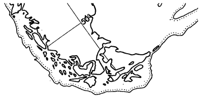
FIGURE 5. The fit of Africa and South America Mercator's projection. Over
