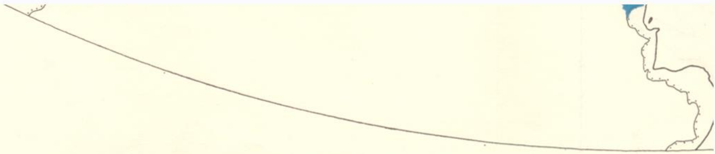
FIGURE 7. The fit of North America, Greenland and Europe at the 500 fm. contour
