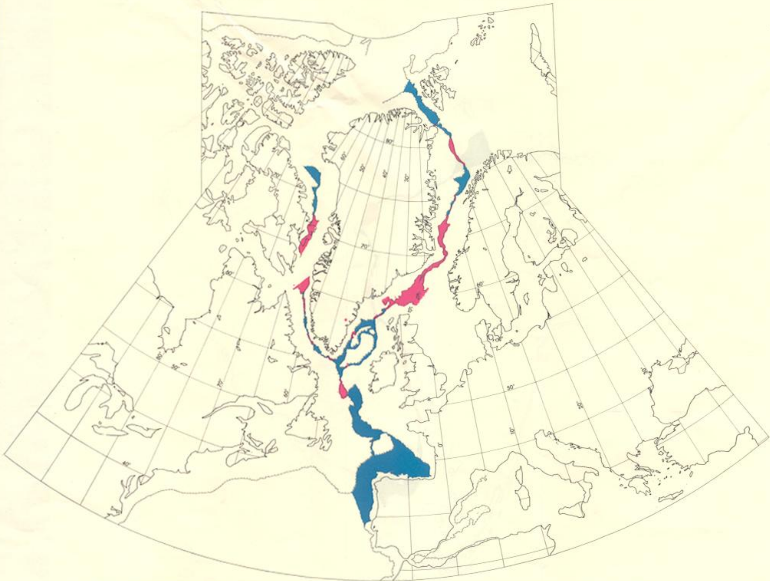
FIGURE 7. The fit of North America, Greenland and Europe at the 500 fm. contour (fits 1 and 2 of table 2), conical projection. Overlaps in red, gaps in blue.
