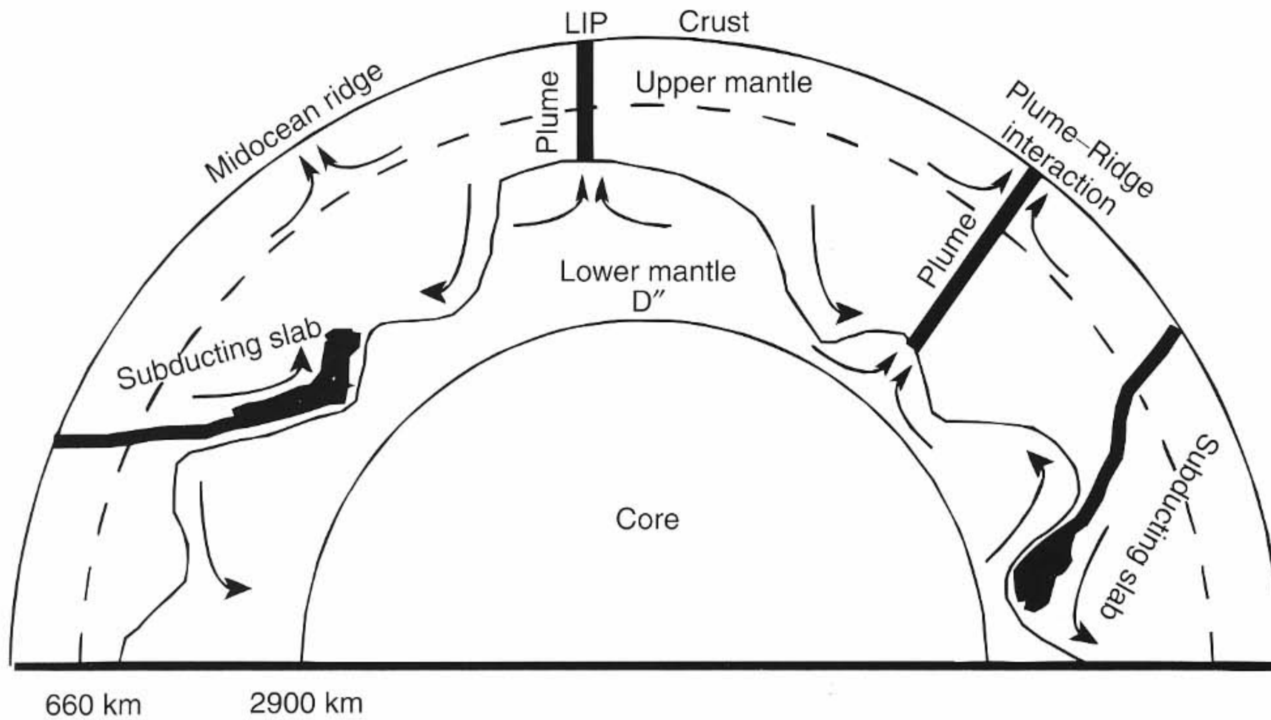
Figure 3 Model of the Earth's interior showing plumes, subducting slabs, and two mantle layers that move in complex patterns, but never mix.
