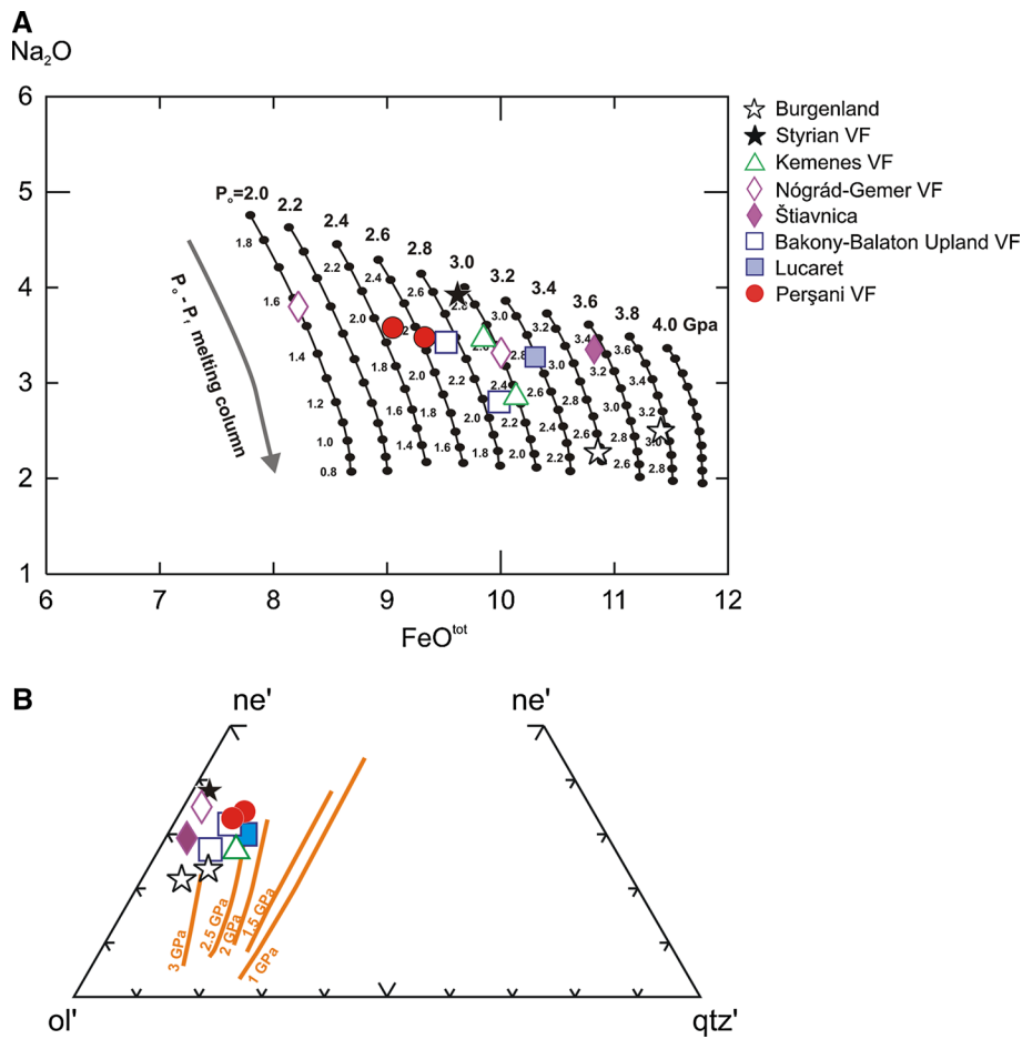
Fig. 6 a Estimation of the initial and final pressures ( p_0 and p_f , respectively) of the melting column for selected CPR basalts using the adiabatic decompression model of Langmuir et al. (1992). The FeO I and the Na 2 O of the calculated primary magmas of the CPR basalts yield information on the initial melting pressure and the cessation of the melting, i.e., the final melting pressure. Each curve represents polybaric mantle melting lines with different initial melting pressure, i.e., where the ambient mantle temperature intersects the
