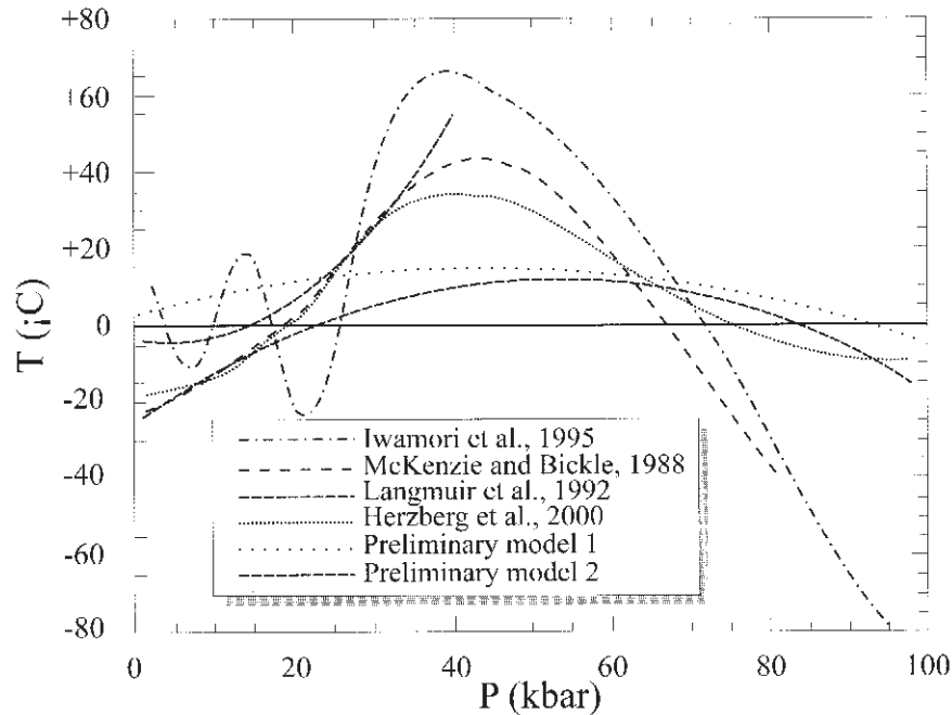
Fig. 3 – Comparison of recommended peridotite solidus of Hirschmann (2000) relative to other selected models of peridotite solidi from literature. Recommended solidus results from peridotite data, with exclusion of enriched and depleted compositions. Positive values of plotted parameter indicate temperatures hotter than Hirschmann's (2000) proposed best-fit model. Preliminary models 1 and 2 are solidi obtained by Hirschmann (2000) using entire range of experimental results from literature, not filtered for enriched and depleted compositions, and the solidi obtained excluding MORB-pyroxite and similar compositions, respectively. For a complete list of references, see Hirschmann (2000).
