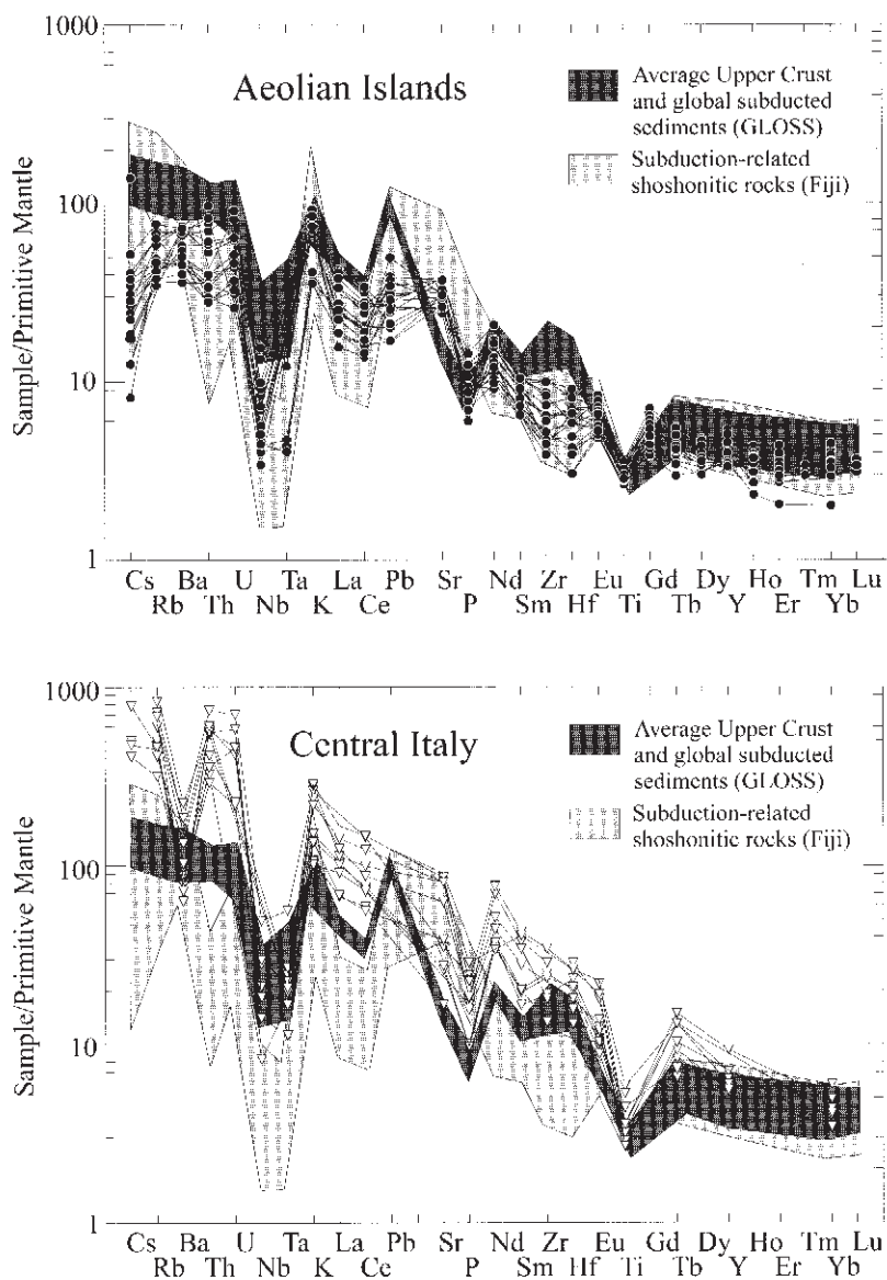
Fig. 1 -- Primitive mantle (Sun and McDonough, 1989) normalized diagram for selected Pliocene to Present Italian mafic volcanic rocks (references in Lustrino, 2000b). Heavy shaded field = upper crust estimates (Wedepohl, 1995; Gao et al. , 1998a) and GLOSS composition (GLOSS = GLOBal Subducting Sediments; Plank and Langmuir, 1998); light shaded field = typical shoshonitic volcanic and plutonic rocks from subduction-related setting (Tavua volcano, Fiji; Rogers and Seatterfield, 1994). Pliocene to present Italian mafic volcanic rocks display typical trace element features of both subduction-related magmas and upper crust. Simple bulk mixing between N-MORB mantle-like composition and upper crustal composition has been ruled out on geochemical modelling grounds by several authors (e.g., Conticelli and Peccerillo, 1992). Instead, for Italian rocks, an origin from mantle sources metasomatized by slab-derived fluids/melts is preferred. The origin of these modifications has been related either to ancient processes or to coeval (Miocene to Present) subduction processes responsible for the opening of the Tyrrhenian sea as a back-arc basin.
