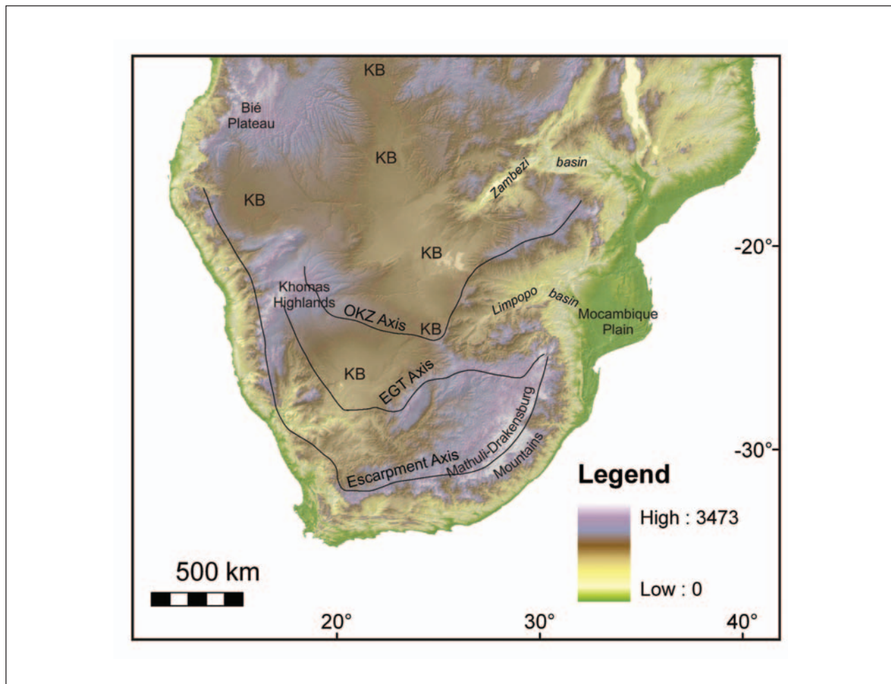
Figure 1. SRTM digital elevation image for southern Africa. The highest elevations are associated with the marginal escarpment and the central Zimbabwe watershed. This high ground surrounds the Cenozoic sediments in the Kalabari Basin (KB). EGT = Etosha-Griqualand-Transvaal Axis; OKZ = Ovambo-Kalabari-Zimbabwe Axis. Elevations in metres.
