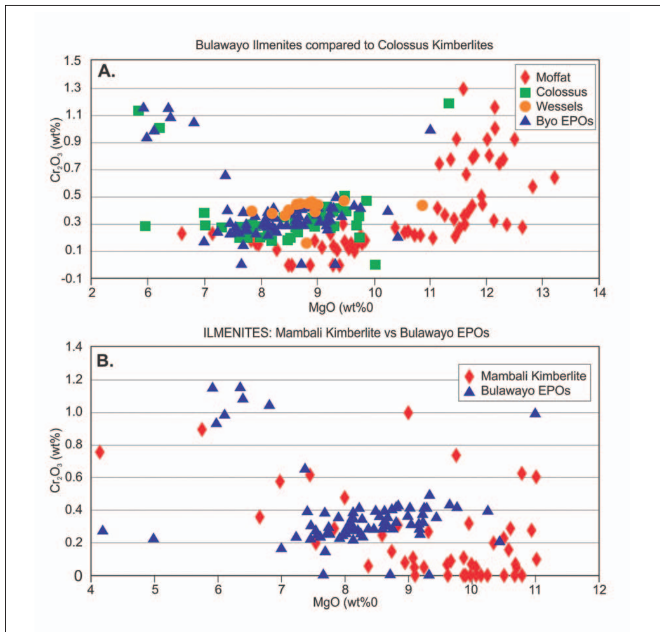
Figure 7. (a) Comparison of chemical fields for ilmenites from the Bulawayo Block and kimberlites from the Colossus cluster. Sources of Data: Bulawayo Block: Moore, 1998a; b; Colossus, Moffat and Wessels: Hildebrand (1993). (b) Comparison of chemical field for ilmenites from the Bulawayo Block and Mambali kimberlite, southwestern Zimbabwe. Sources of data: Bulawayo Block: Moore, 1998 a; b; Mambali kimberlite: Data for the Mambali kimberlites kindly provided by Leon Daniels.
