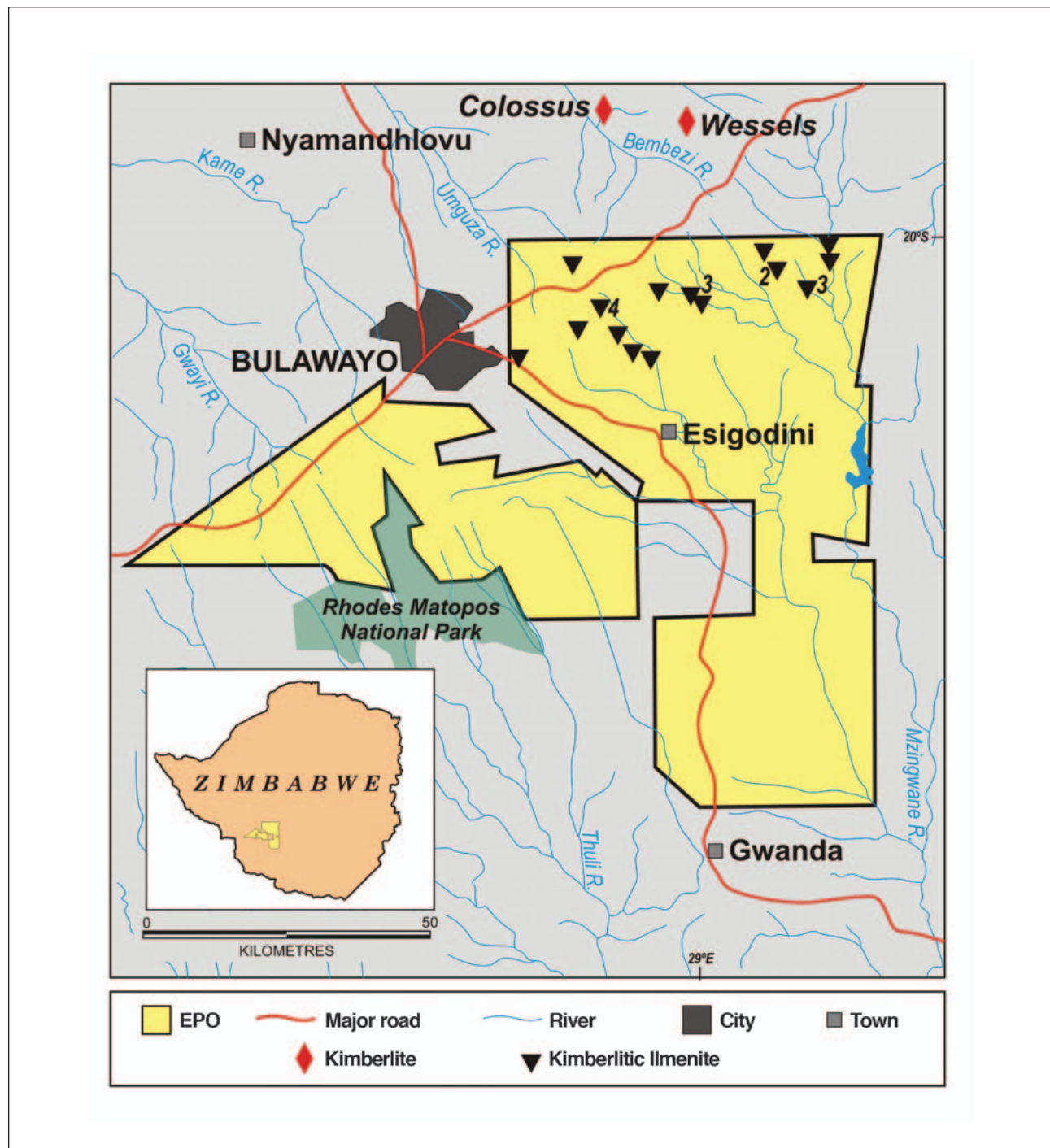
Figure 3. Detail of the Bulawayo Block in relationship to the drainage system. Inverted triangles denote the sites of samples in which kimberlitic ilmenites were recovered. Numbers denote the numbers of >500µm ilmenites if more than one grain was present. Data from Moore (1998a; b).
