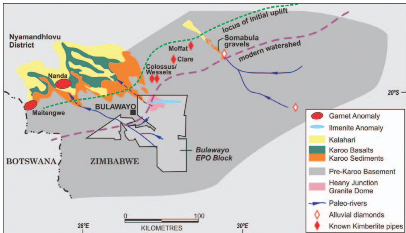
Figure 2. Location of the Bulawayo EPOs in relationship to a simplified regional geology and the modern watershed (long-dashed lines) between the Zambezi and Limpopo drainage basins. Short-dashed line shows inferred initial locus of epeirogenic flexure, located to the north of the modern watershed
