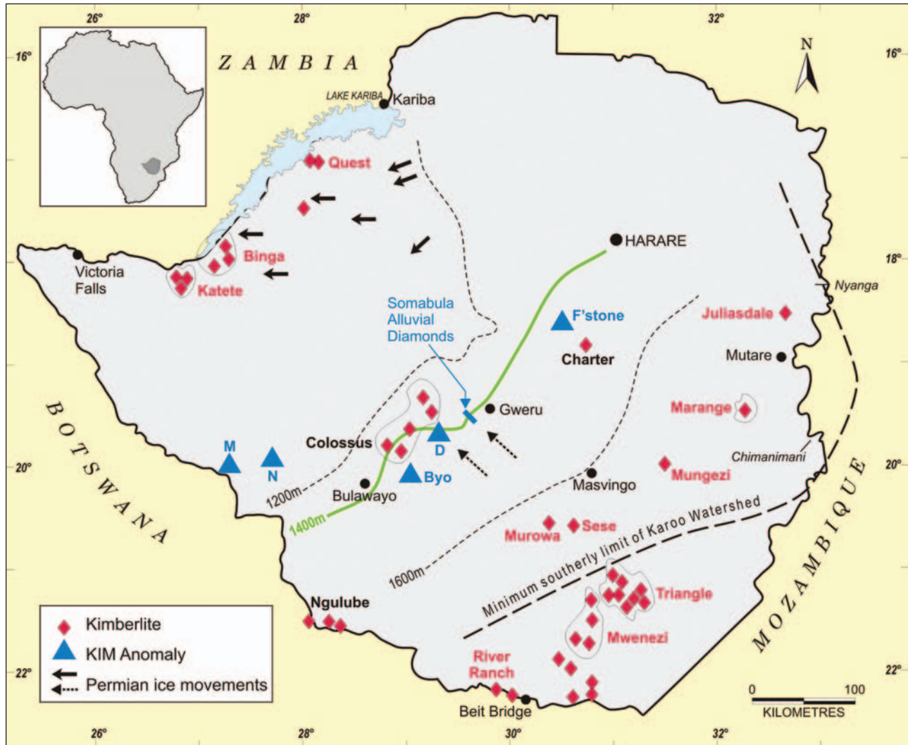
Figure 4. Locations of known kimberlite clusters in Zimbabwe. Light-dashed and solid lines denote elevations in metres on the pre-Karoo surface (from Lister, 1987). The solid line (1400 m) lies close to the modern watershed. Bold dashed line showing the minimum southerly limit of the Karoo watershed is from Moore et al., 2009b. Triangles denote unexplained kimberlitic heavy mineral anomalies. M = Maitengue; N = Nanda; Byo = Bulawayo Block; D = Daiseyfield (From Moore et al., 2009b). Solid black arrows show inferred Permian ice movements summarized by Lister (1987); Dashed black arrows show Permian ice movements inferred by Moore and Moore (2006).
