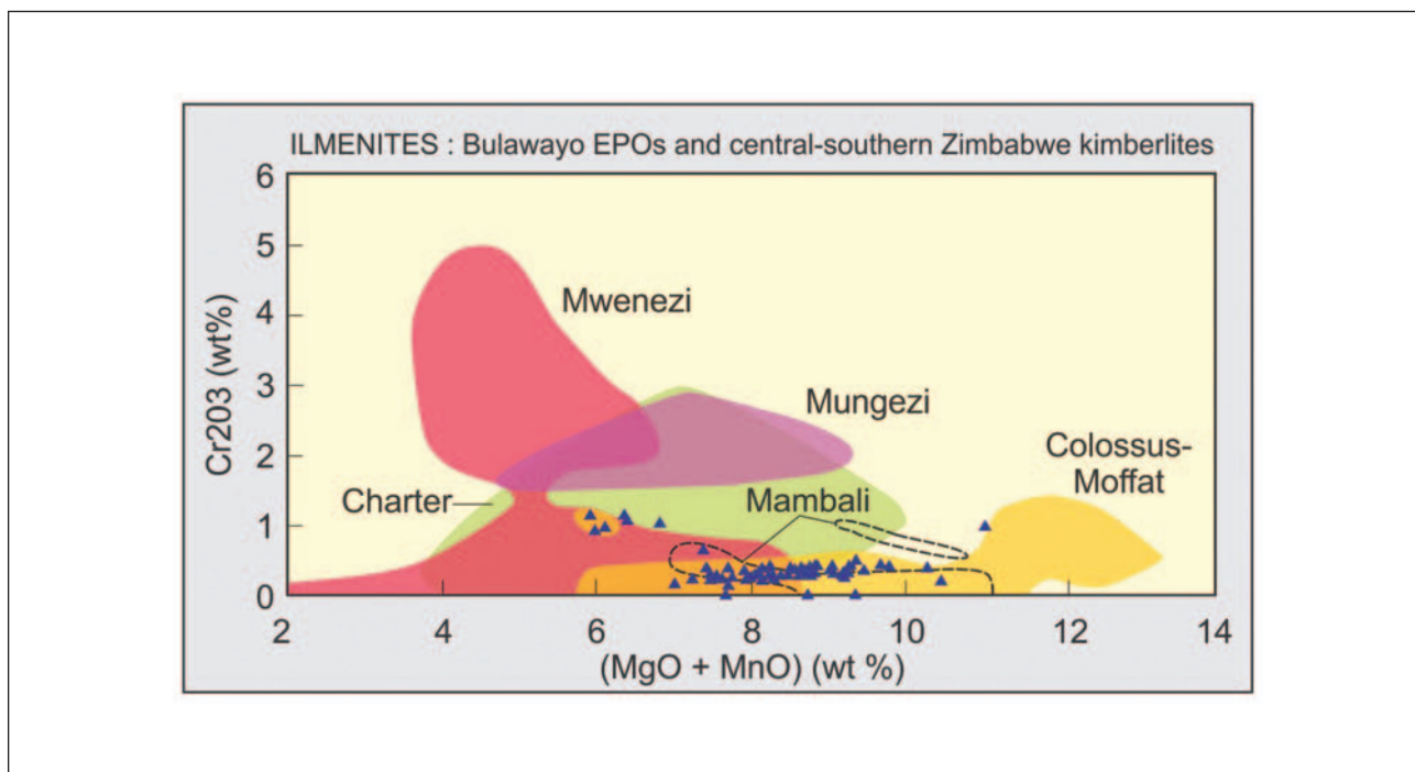
Figure 6. Compositional fields for picroilmenites from kimberlites in south and central Zimbabwe in relationship to compositions of those from the Bulawayo Block (triangles). Sources of Data: Bulawayo Block: Moore, 1998a; b; Charter Kimberlite: Brennan, 1999; Colossus-Moffat: Hildebrand, 1993; Mambali: Data kindly provided by Leon Daniels; Mungezi: Kimberlitic Searches (Pty.) Ltd/Somabula Explorations (Pty.) Ltd. Joint Venture, in house data; Mwenezi: Williamson and Robey, 1999.
