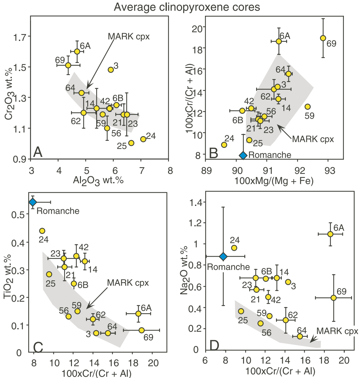
Figure 8. Average compositions and standard deviation of clinopyroxene porphyroclast cores for each dredges. Same legend as Figure 6. In addition, blue diamond are spinel-hercynites from the Romanche Fracture Zone, Atlantic ocean [Seyler and Bonatti, 1997].
