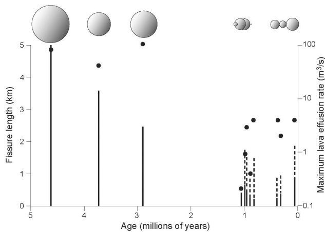
Figure 2. Plot of eruptive volume (circles sized in proportion to cube-root of volume) fissure length (lines), and lava effusion rate (dots) for Pliocene-Pleistocene volcanoes of the Southwestern Nevada Volcanic Field. Note that age determinations do not allow discrimination of relative ages amongst the five Pleistocene volcanoes in Crater Flat, therefore they plotted in random order around 1 Ma. The eruptive products of SW and NE Little Cones are largely buried by alluvium and mapped by aeromagnetic anomaly [Valentine et al. , 2006]; their volumes are lumped together in this plot.
