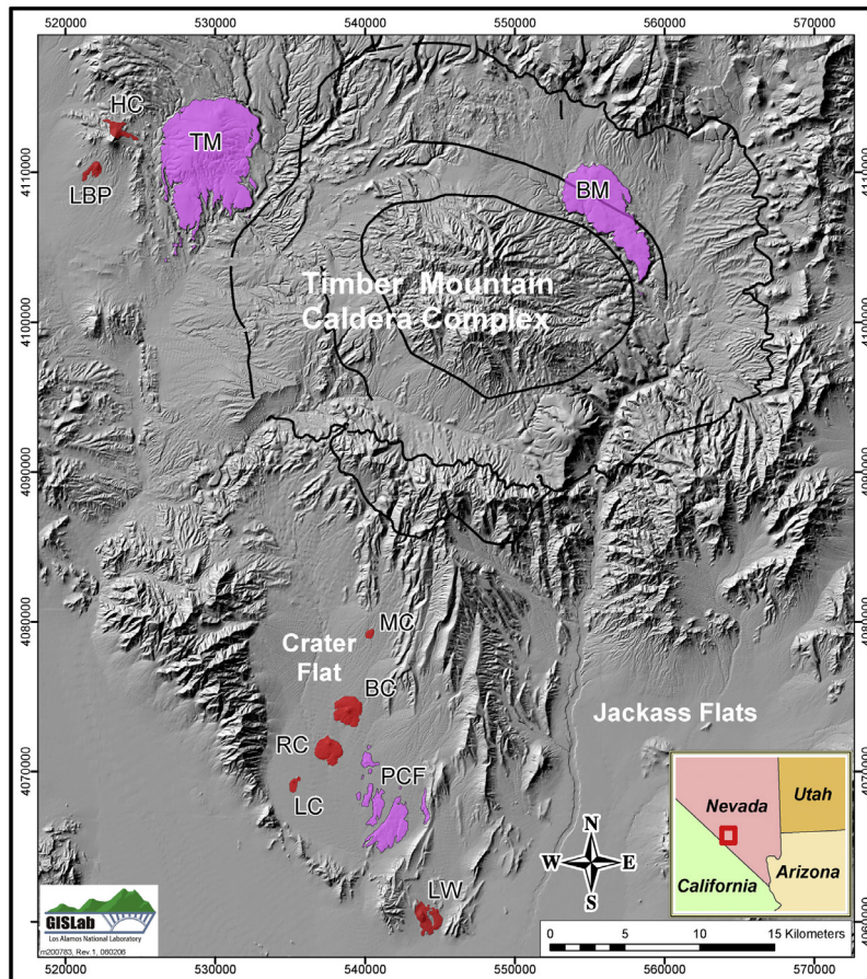
Figure 1. Digital elevation model (DEM) showing distribution of Pliocene-Pleistocene basaltic volcanoes in the Southwestern Nevada Volcanic Field (not including known or inferred buried volcanoes). Pliocene volcanoes (magenta) include Thirsty Mountain (TM), Pliocene Crater Flat (PCF), and Buckboard Mesa (BM). Pleistocene volcanoes (red) include Makani (MC), Black Cone (BC), Red Cone (RC), SW and NE Little Cones (both labeled together as LC), Little Black Peak (LBP), Hidden Cone (HC), and Lathrop Wells (LW). Solid lines represent margins of Miocene silicic calderas [Wahl et al. , 1997]. Crater Flat and Jackass Flats are major structural basins (note that most linear ridges and range fronts in the DEM coincide with normal faults). Inset shows location with respect to the southwestern United States.
